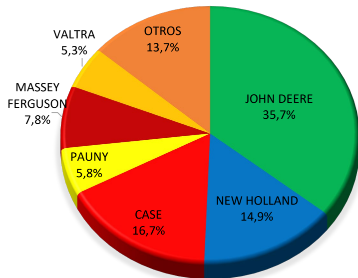
Market Share
